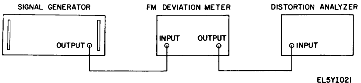
FIG 9-II. TEST SETUP, FM DISTORTION
