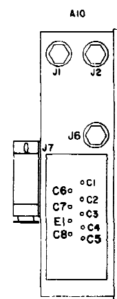
VIEW B-B
